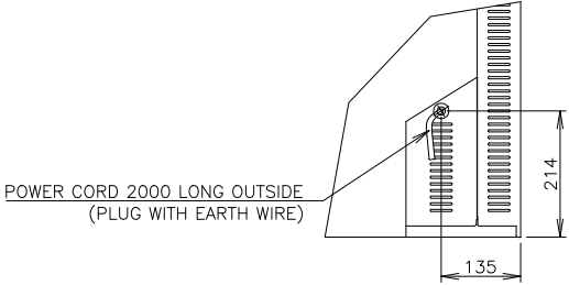
VIEW A(1/10)
